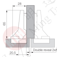
Centre stop
