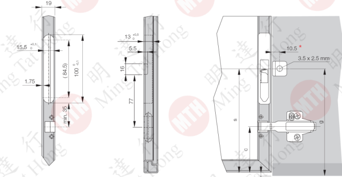
Fitting dimensions
