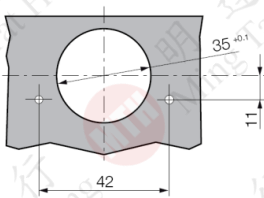
Corner stop
