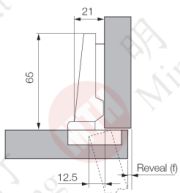
Corner stop
