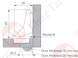
Inset stop
