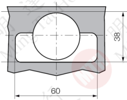
Inset stop
